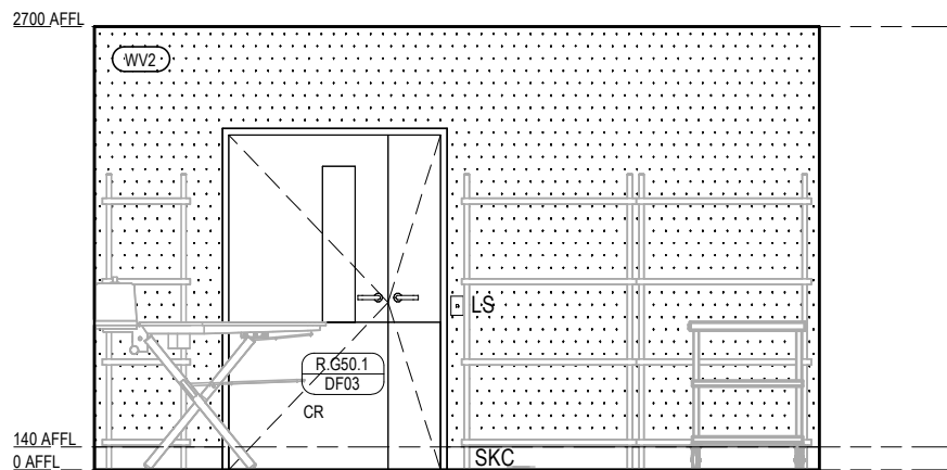
LAUNDRY SIDE 2 ELEVATION 1 Scale 1 : 50
