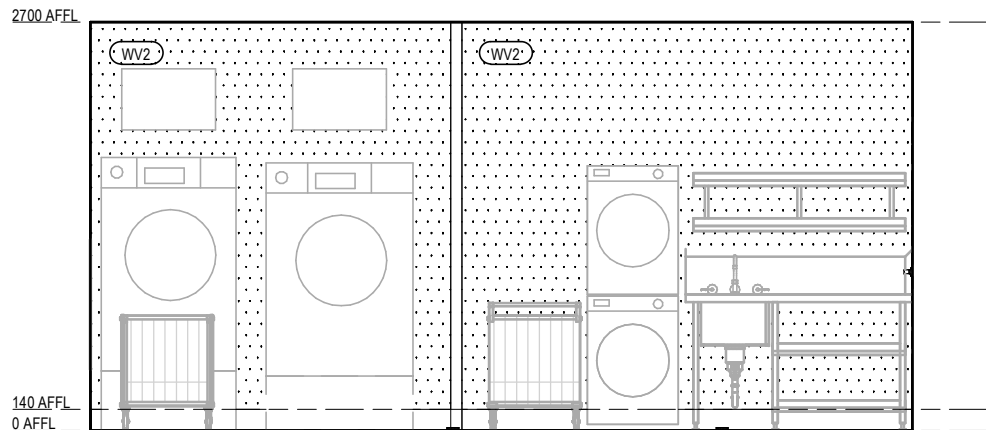
LAUNDRY SIDE 1 ELEVATION 4 Scale 1 : 50
