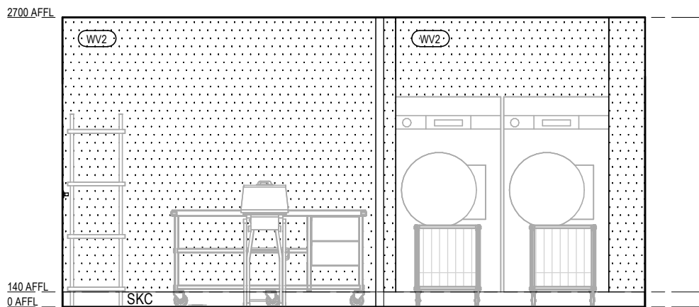
LAUNDRY SIDE 2 ELEVATION 2 Scale 1 : 50
