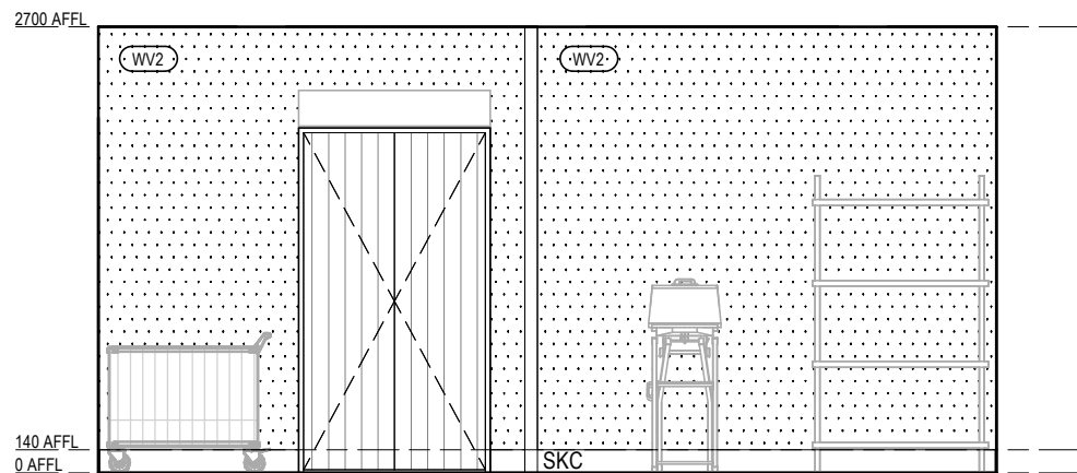
LAUNDRY SIDE 2 ELEVATION 4 Scale 1 : 50
