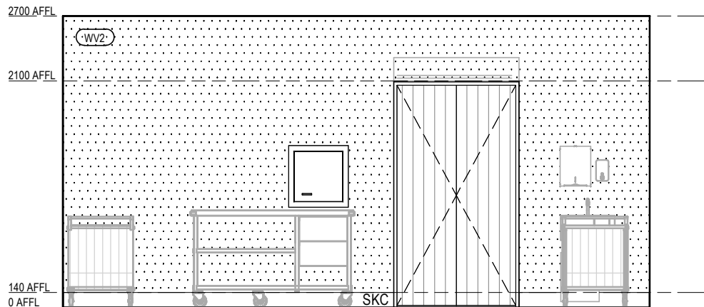
LAUNDRY SIDE 1 ELEVATION 2 Scale 1 : 50
