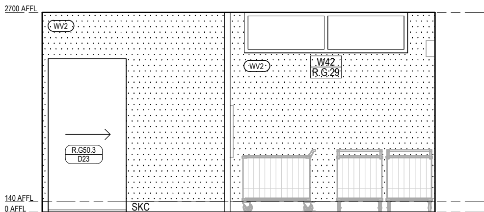
LAUNDRY SIDE 2 ELEVATION 3 Scale 1 : 50
