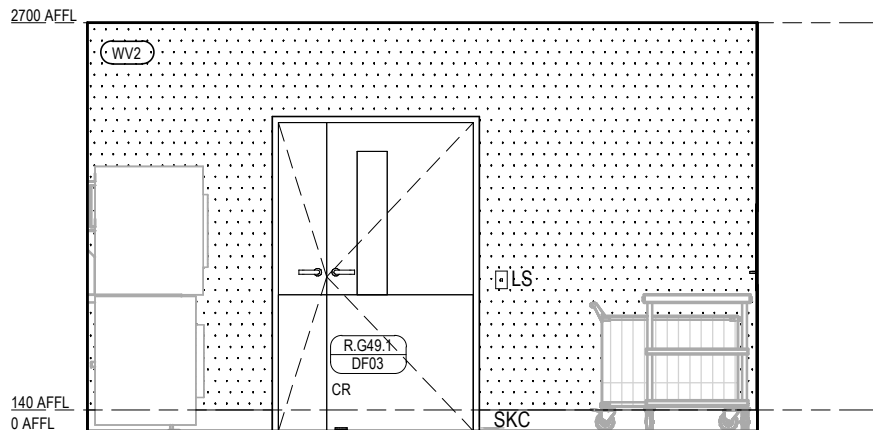
LAUNDRY SIDE 1 ELEVATION 1 Scale 1 : 50
