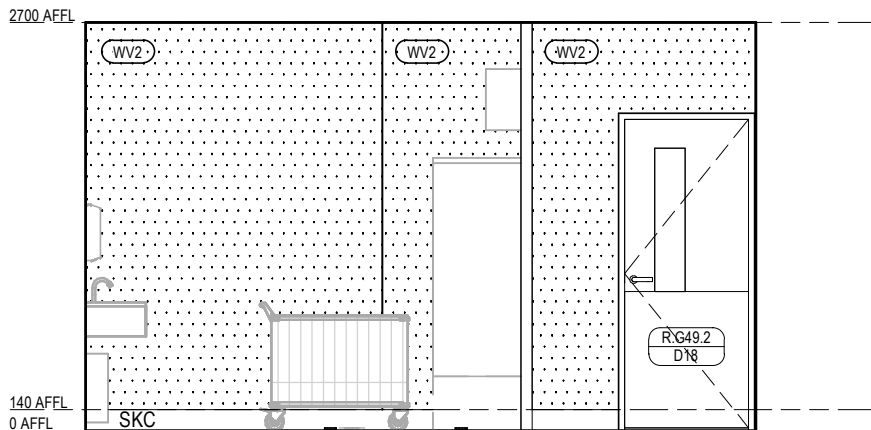
LAUNDRY SIDE 1 ELEVATION 3 Scale 1 : 50
