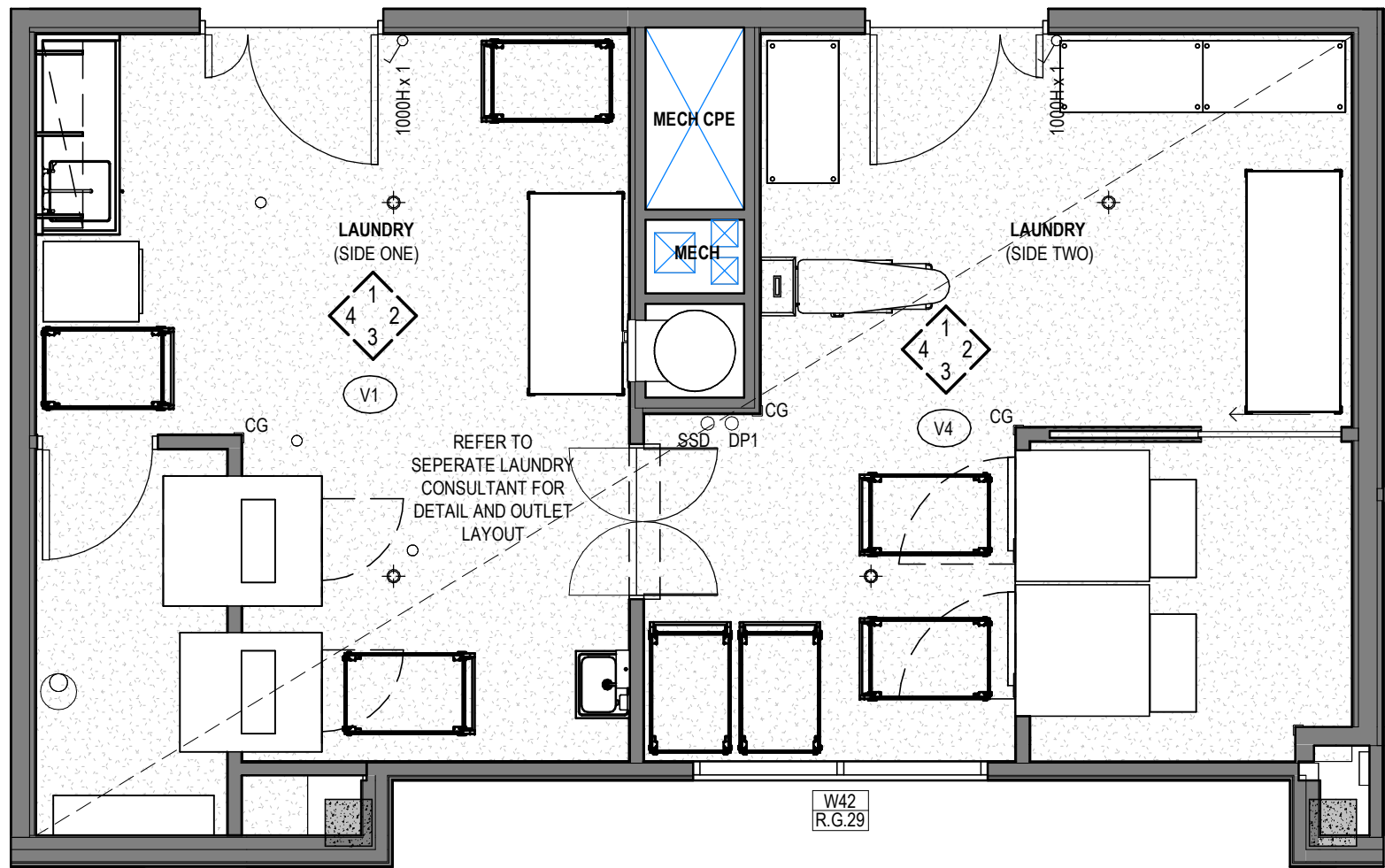
1 LAUNDRY Scale 1 : 50
